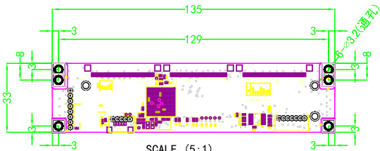
SCALE (5:1) EETI EXC80H100 Controller
